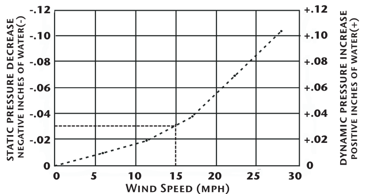
Figure 2: Pressure distribution for an 8" Vacu-Stack® installation
