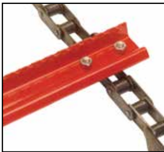
Standard 3/16" Special lip design increases strength and rigidity reducing breaking and bending.
