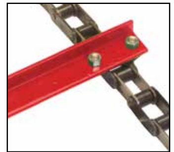
T Slat Same material as original and bolted to the chain.
