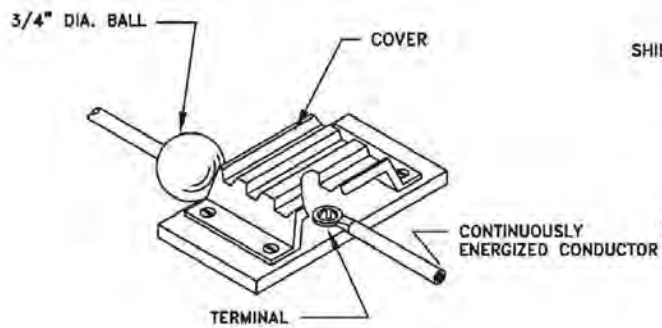
INSULATED COVER
