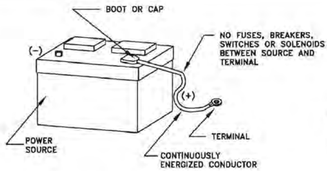
CONTINUOUSLY ENERGIZED TERMINAL
