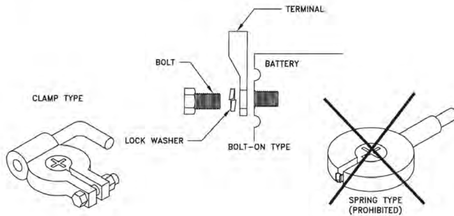
FIGURE 17 Battery Terminal Connections
