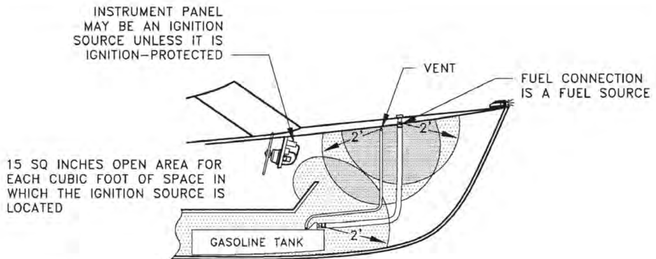
FIGURE 8c Isolation of Electrical Components
