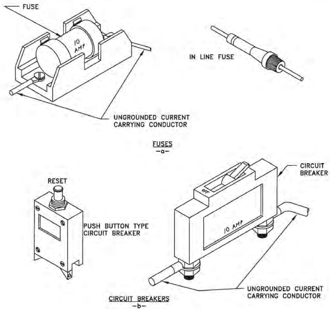
FIGURE 23 OVERCURRENT PROTECTION
