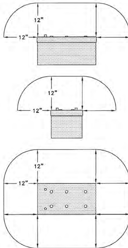
FIGURE 15 Dielectric Shielding Envelope
