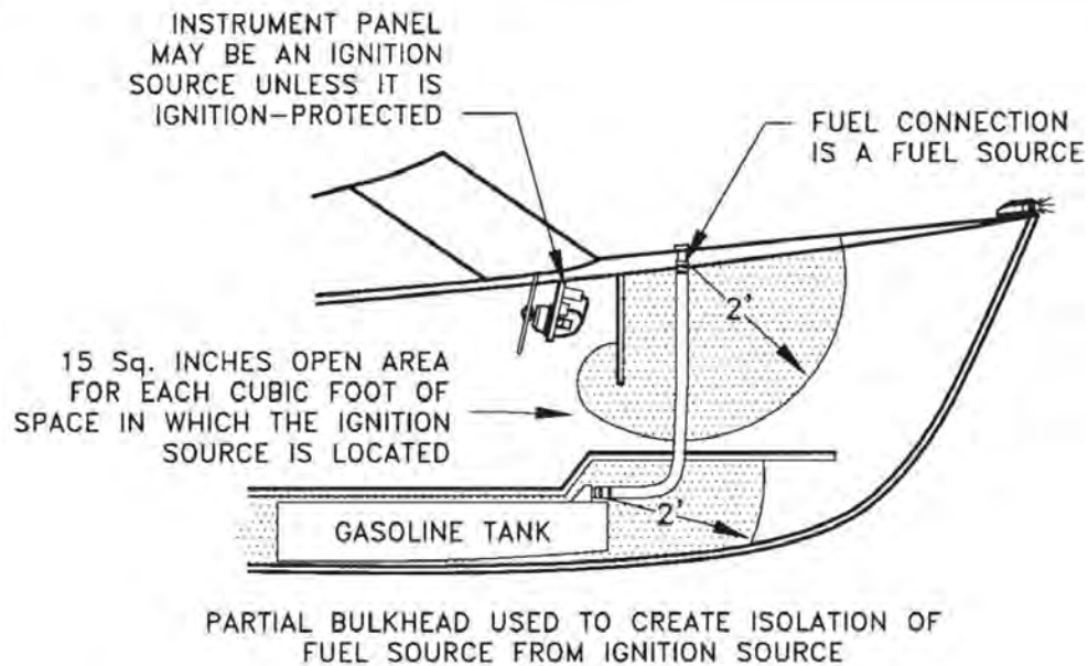
FIGURE 8b Isolation of Electrical Components
