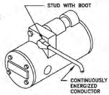
INSULATED BOOT, NIPPLE OR CAP
