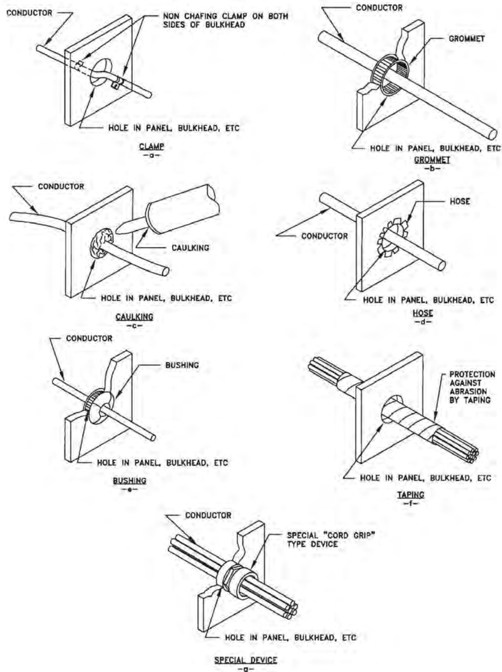
FIGURE 21 - Abrasion Protection
