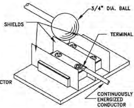
SHIELD
