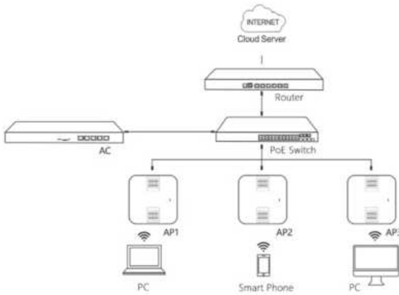
Connection Diagram 1
