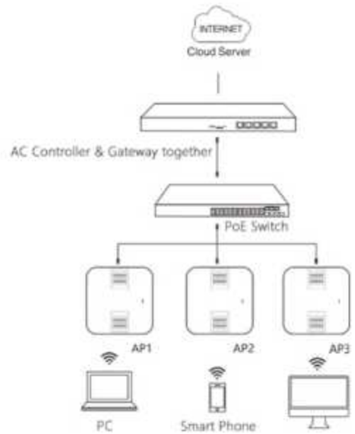
Connection Diagram 2
