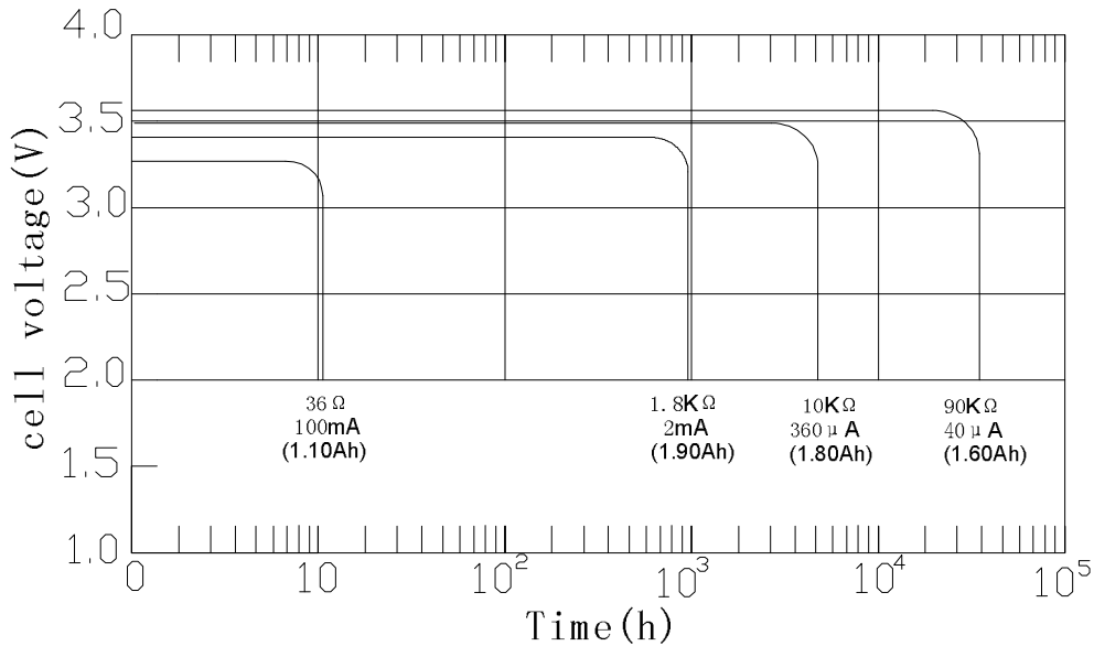
Discharge performance
