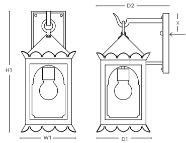
DIMENSIONS SBLC-40-AM
