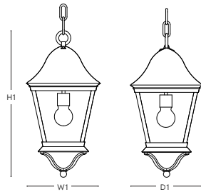
DIMENSIONS SBLC-23B-PD
