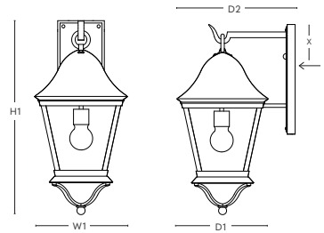
DIMENSIONS SBLC-23B-AM
