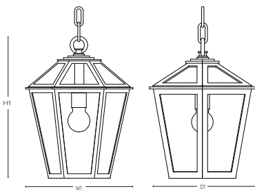
DIMENSIONS SBLC-5B-PD
