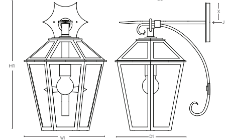
DIMENSIONS SBLC-5B-AM
