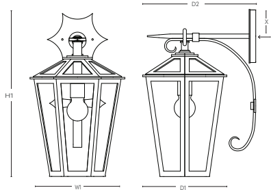
DIMENSIONS SBLC-5B-AM
