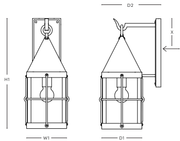
DIMENSIONS SBLC-18A-AM
