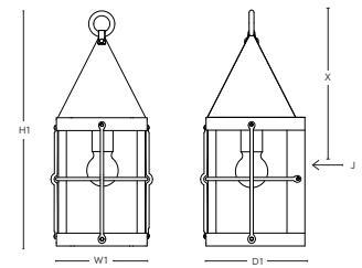
DIMENSIONS SBLC-18A-FM
