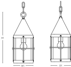
DIMENSIONS SBLC-18A-PD
