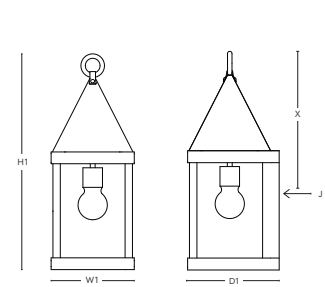
DIMENSIONS SBLC-19-FM
