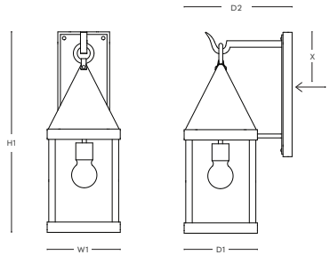
DIMENSIONS SBLC-19-AM
