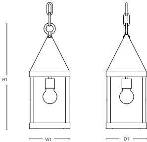
DIMENSIONS SBLC-19-PD
