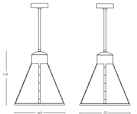
DIMENSIONS SBLC-92-PD
