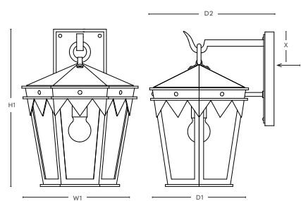
DIMENSIONS SBLC-9-AM
