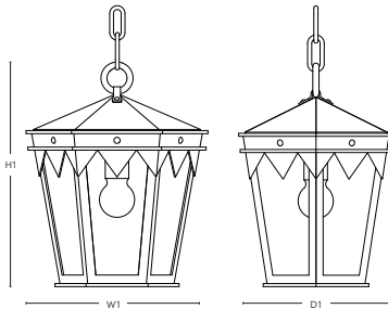
DIMENSIONS SBLC-9-PD
