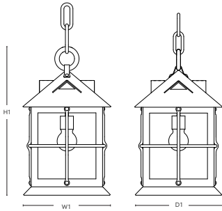
DIMENSIONS SBLC-1B-PD
