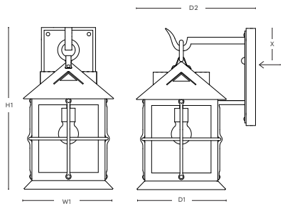
DIMENSIONS SBLC-1B-AM
