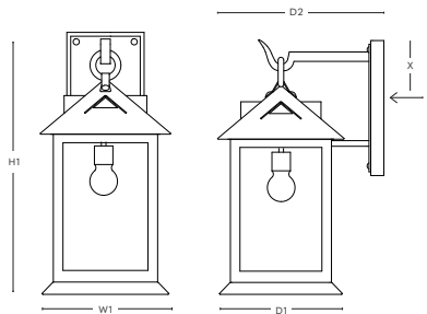
DIMENSIONS SBLC-1A-AM
