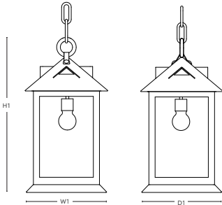
DIMENSIONS SBLC-1A-PD
