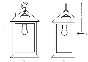
DIMENSIONS SBLC-1A-FM
