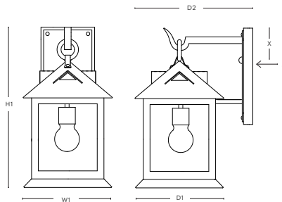
DIMENSIONS SBLC-1A-AM
