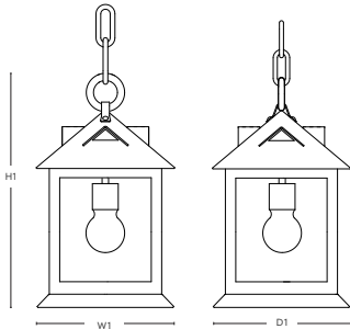
DIMENSIONS SBLC-1A-PD
