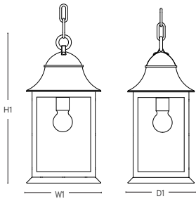
DIMENSIONS SBLC-5B-PD
