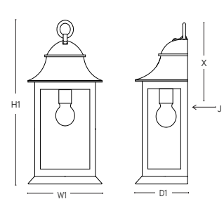
DIMENSIONS SBLC-5B-FM
