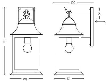
DIMENSIONS SBLC-5B-AM
