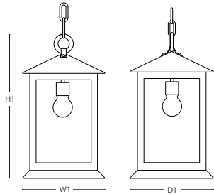
DIMENSIONS SBLC-39-PD
