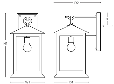
DIMENSIONS SBLC-39-AM
