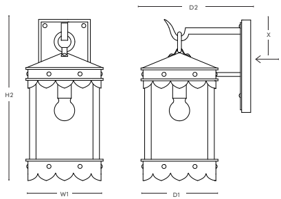
DIMENSIONS SBLC-6ASB-AM
