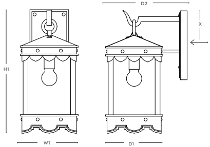
DIMENSIONS SBLC-6A-AM
