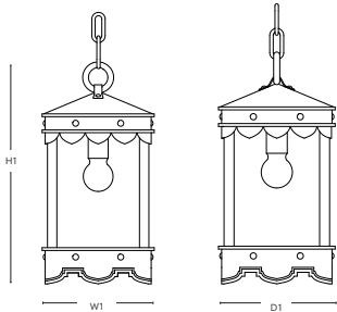
DIMENSIONS SBLC-6A-PD
