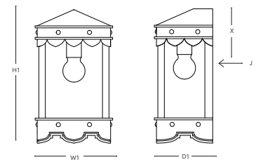
DIMENSIONS SBLC-6A-FM
