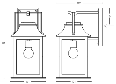
DIMENSIONS SBLC-20B-AM
