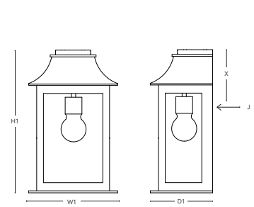
DIMENSIONS SBLC-20B-FM
