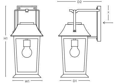
DIMENSIONS SBLC-16A-AM
