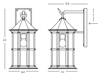
DIMENSIONS SBLC-16A-AM
