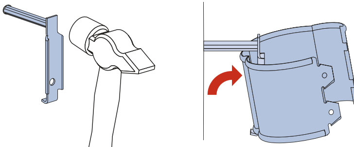
Drive-in fixing
