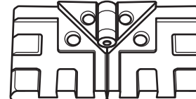
GGH2-B Two Panel Connector Hinging
