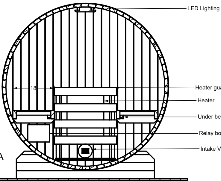
SECTION C-C SCALE 1:25
