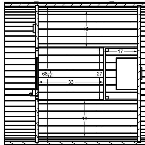
SECTION C-C SCALE 1:25
