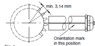
Fig. 1 Accurate mounting position
