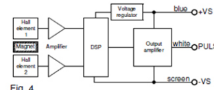
Fig. 4 Circuit diagram
