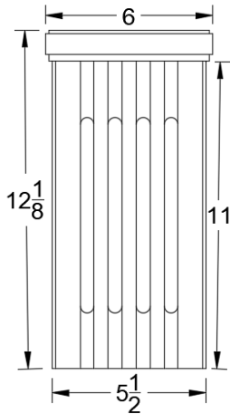
Front Elevation
