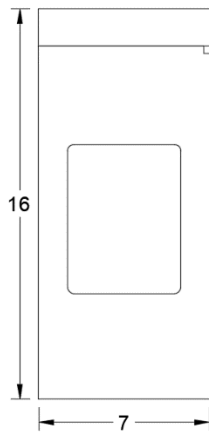
Side Elevation
