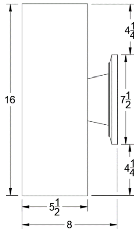
Side Elevation
