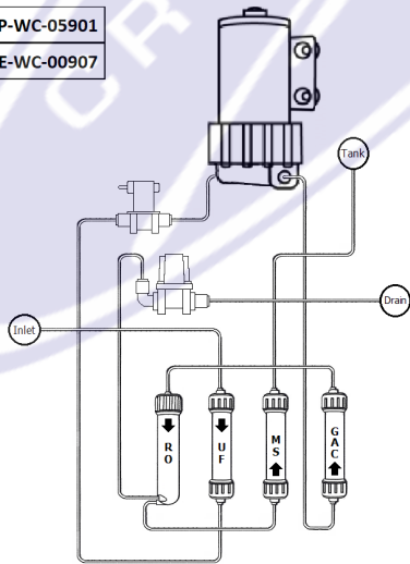
Hybrid RO/UF
