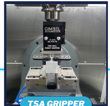
TSA GRIPPER
