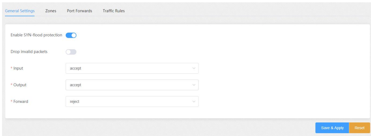
Figure 3.5.4-1 Firewall
