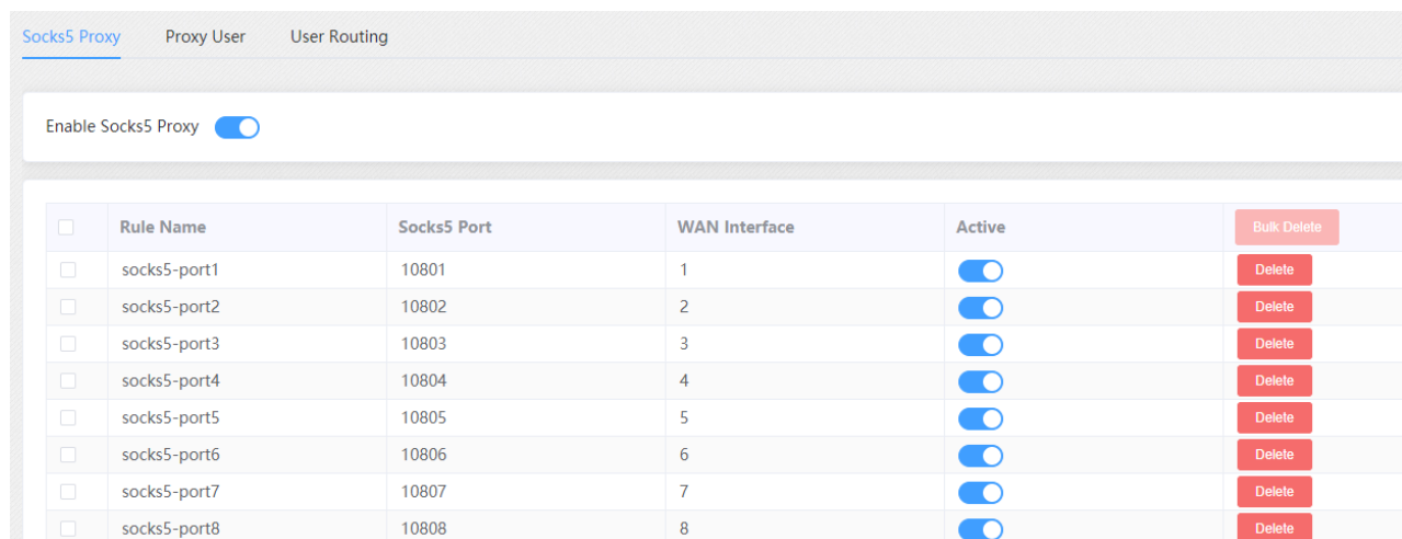
Figure 3.6.1-1 Socks5 Proxy
