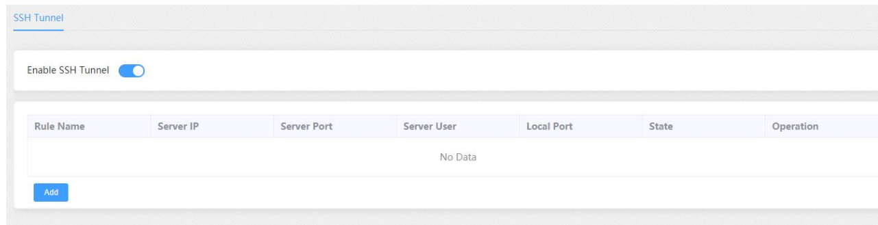
Figure 3.6.3-1 SSH Tunnel
