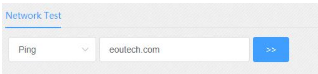
Figure 3.2.4-1 Network test
