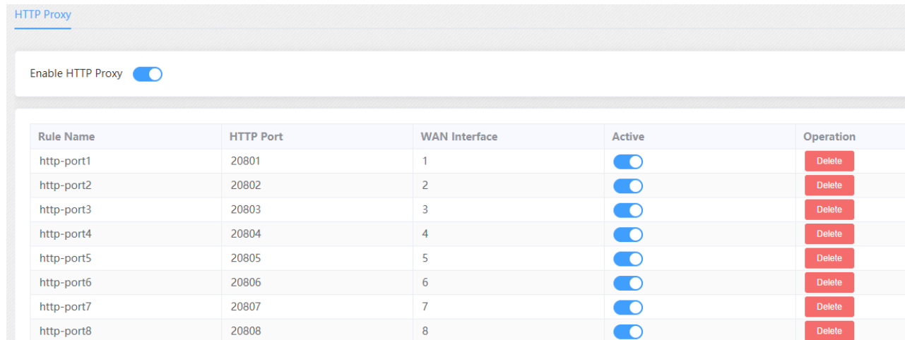
Figure 3.6.2-1 HTTP Proxy
