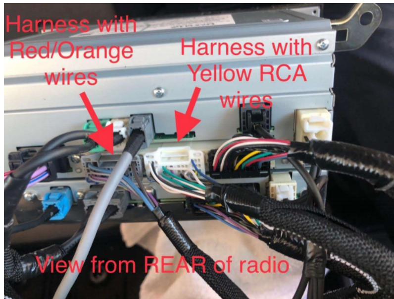
Figure 5 - Rear of 2020+ Radio
