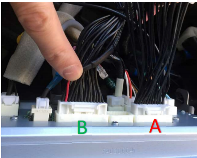
Figure 4 - Override & Video Harnesses Installed (View of radio from top down)
