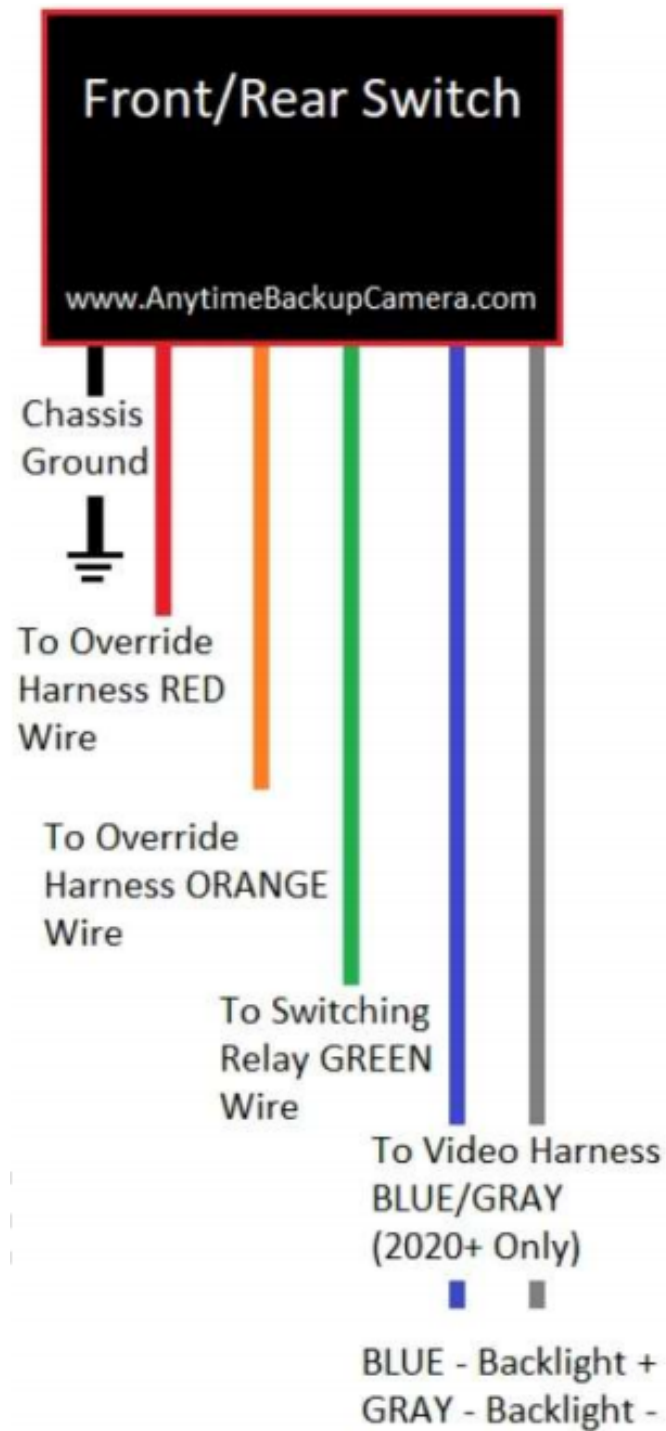
Figure 9 - Front/Rear Switch Wire Descriptions
