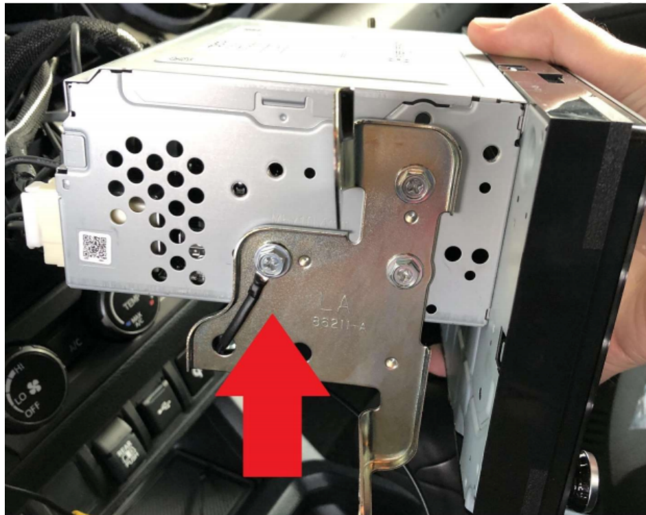
Figure 8 - Grounding Point for Black Wire
