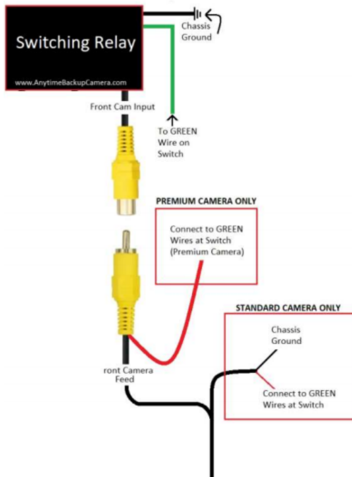
Figure 10 - Front Camera Connections
