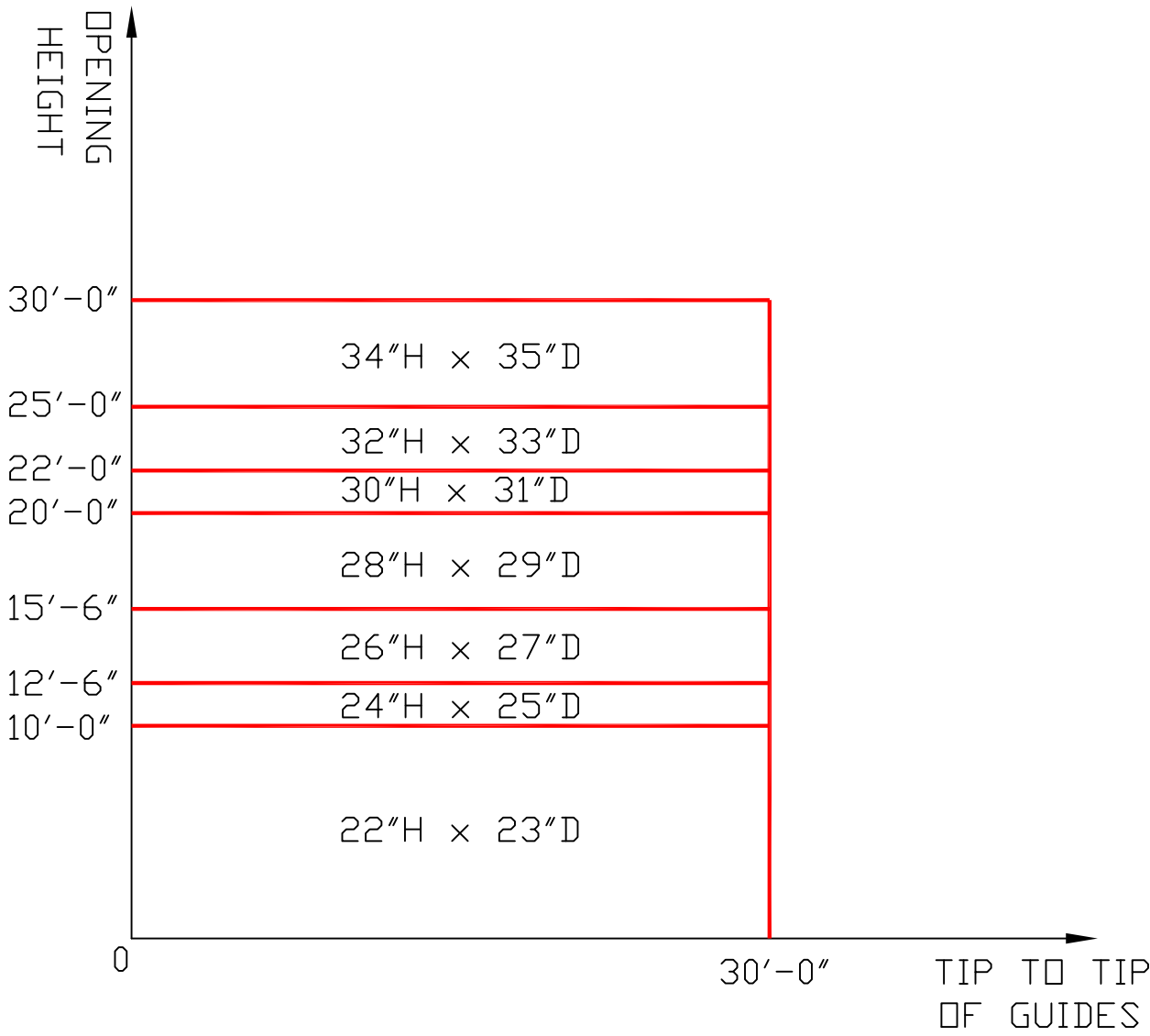
HOOD DIMENSION CHART
