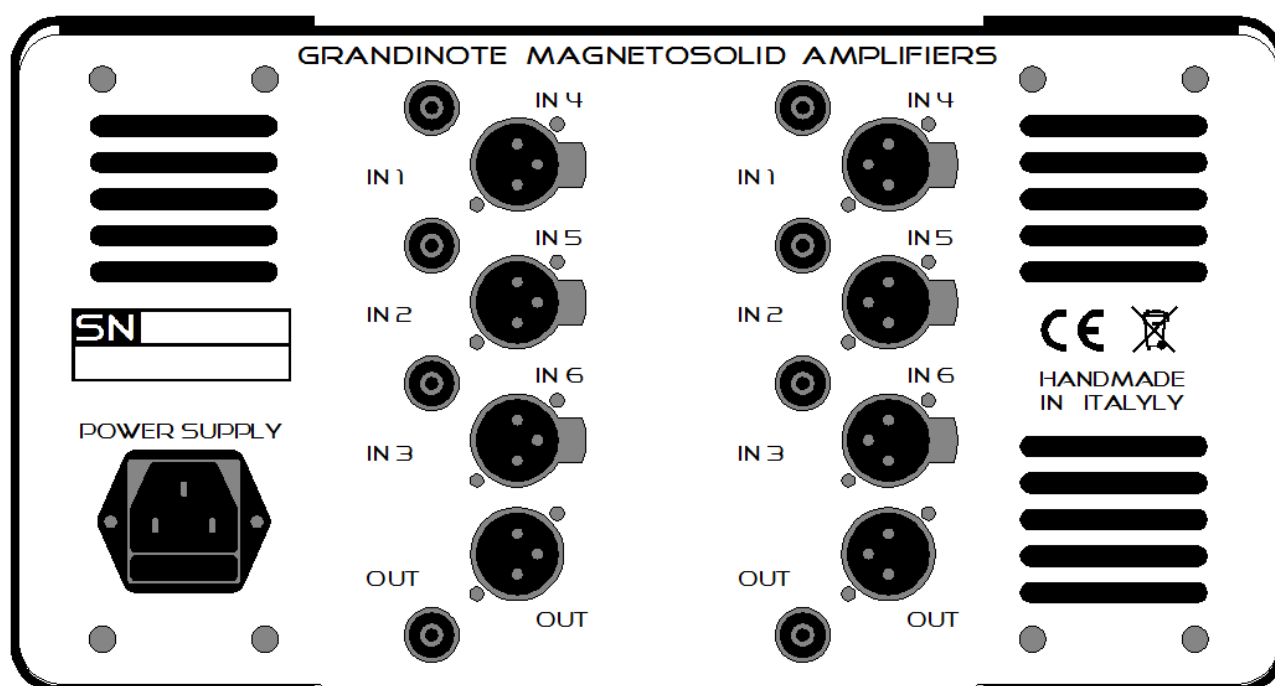
PICTURE 2: REAR PANEL
