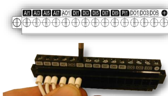
Figure 3. Positive identification on removable terminals
