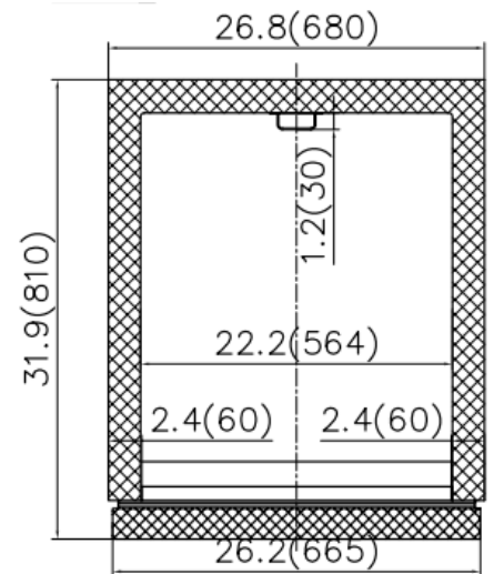
PLAN VIEW
