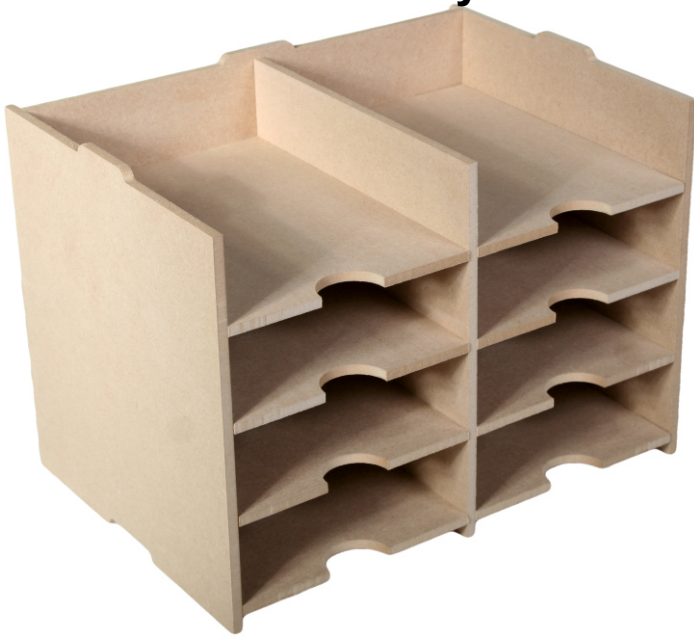
Stacking
