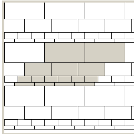
Pattern 5 Pieces per 100 Sqft (2) 900 x 450 = 46%, 12 pcs (3) 600 x 300 = 31%, 12 pcs (6) 300 x 150 = 15%, 36 pcs (4) 451 x 76 = 8%, 24 pcs
