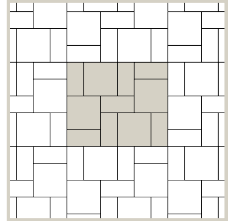
Pattern 3 Pieces per 100 Sqft 300 x 300 = 54%, 56 pcs 300 x 150 = 46%, 126 pcs
