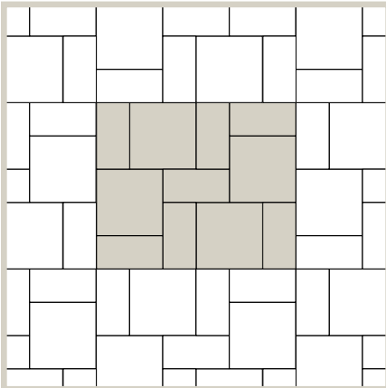
Pattern 4 Pieces per 100 Sqft (1) 900 x 900 = 50%, 6 pcs (2) 900 x 450 = 50%, 12 pcs
