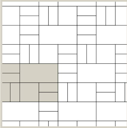
Pattern 1 Pieces per 100 Sqft (6) 150 x 300 = 50%, 102 pcs (1) 300 x 300 = 17%, 17 pcs (1) 600 x 300 = 33%, 17 pcs
