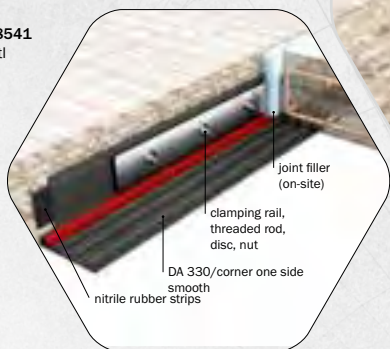
KRASOflex® Clamp Construction - external
