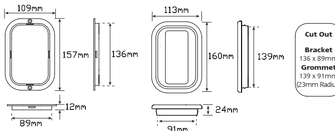
Stop/Tail 130RMC - Single Blister
