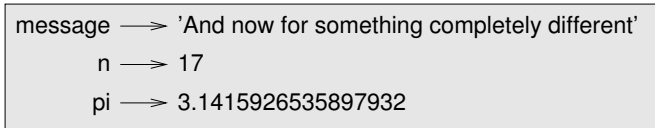
Figure 2.1: State diagram.
