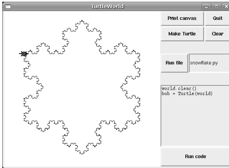
Figure 19.1: Class diagram.
