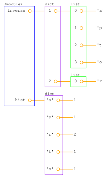
Figure C.4: Object diagram.
