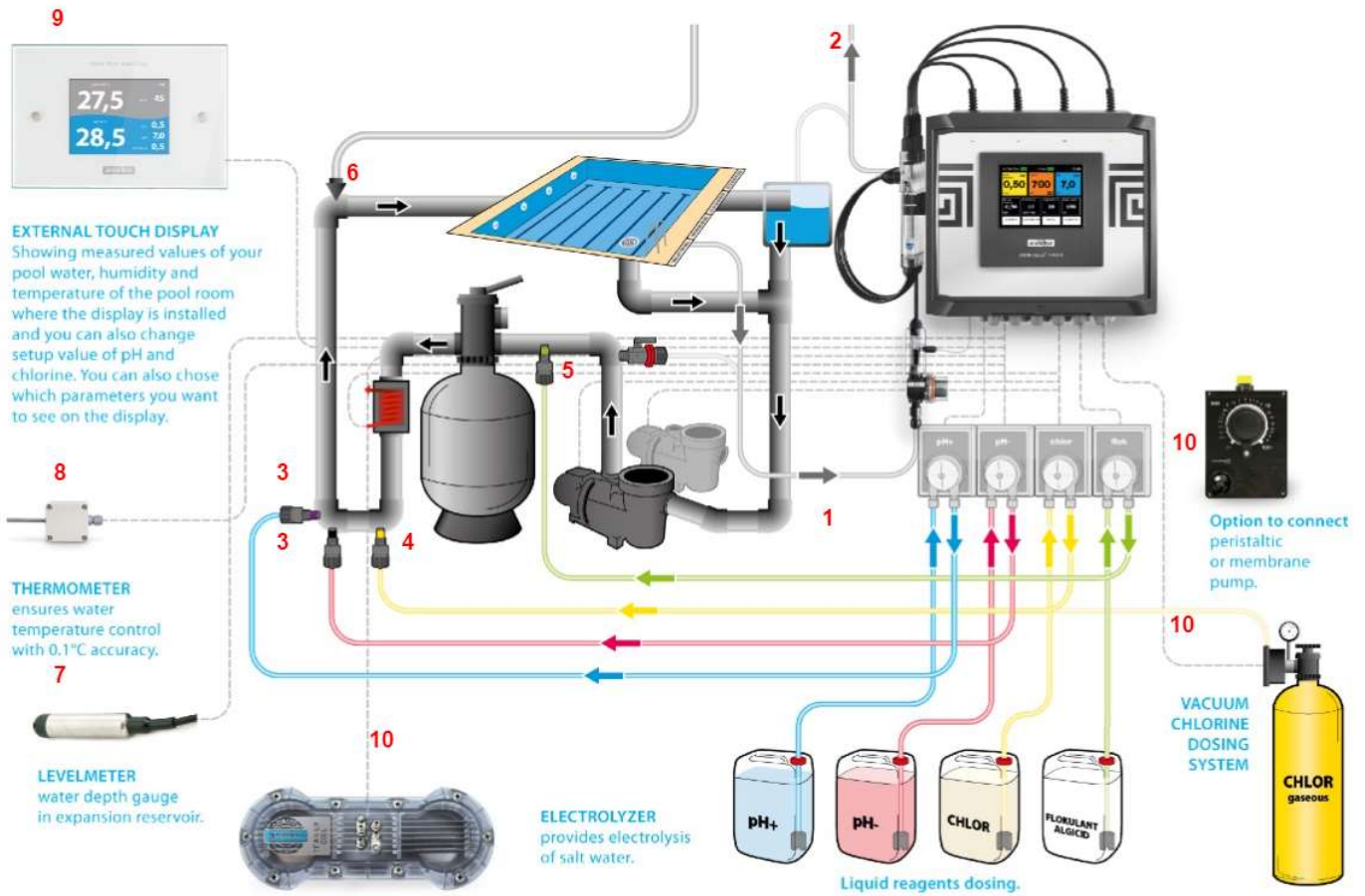
Fig. 1. Connection
