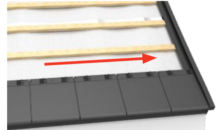
Envirotile Double Tile
