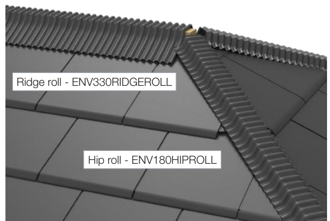
RIDGE ROLL - ENV330RIDGEROLL
