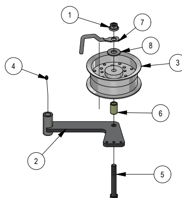
039-6952-23 SD DECK IDLER ASSEMBLY
