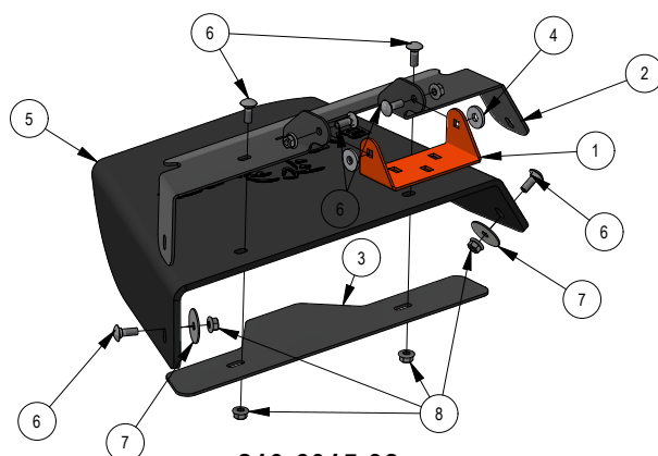
210-6015-98 Discharge Assembly
