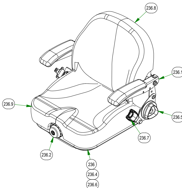
071-6065-22 SEAT ASSEMBLY
