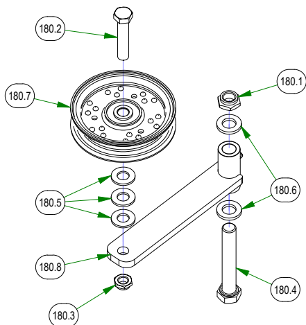
039-0031-19 REAR IDLER PULLEY
