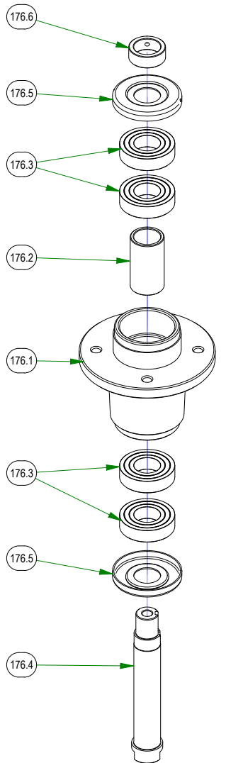
037-4000-00 SPINDLE ASSEMBLY
