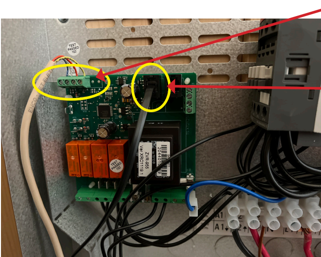
Temperature Sensor
