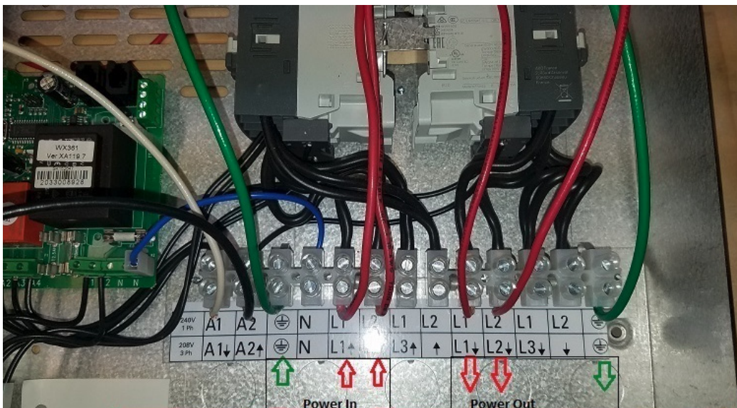
Power Unit Wiring
