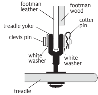
ATTACHING THE FOOTMAN
