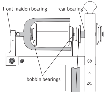
FLYER SHAFT OILING POINTS
