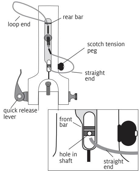
INSTALL THE SCOTCH TENSION BRAKE
