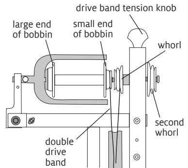
DOUBLE DRIVE MODE
