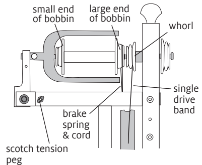
SCOTCH TENSION MODE
