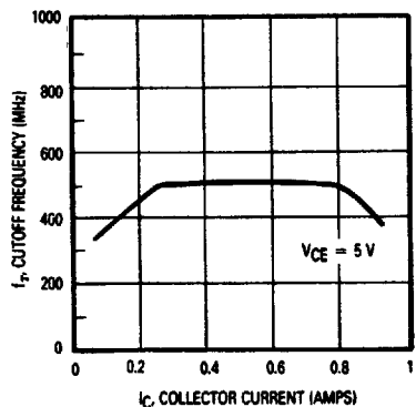
Figure 11. Cutoff Frequency versus Current
