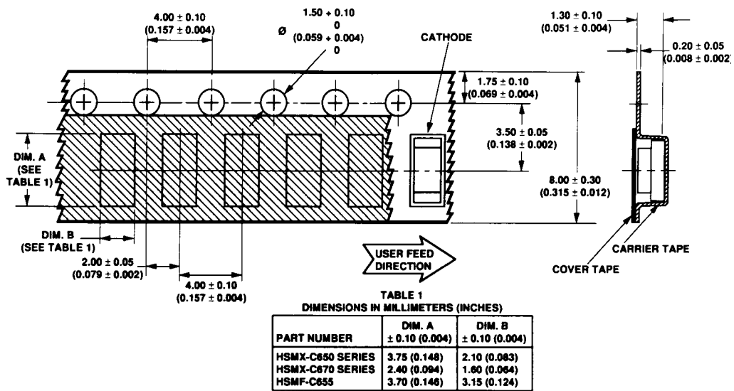
Figure 10. Tape Dimensions.
