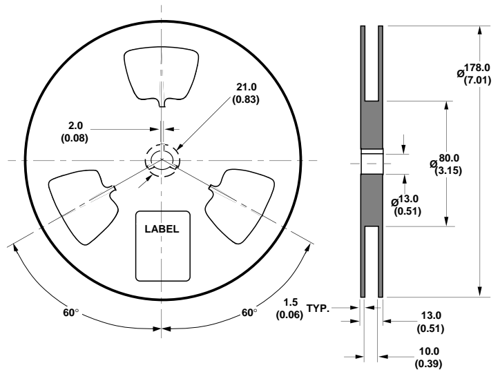
Figure 9. Reel Dimensions.
